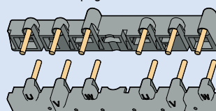
Wire kit, UW for use with Interlock unit ▶ 88 page
