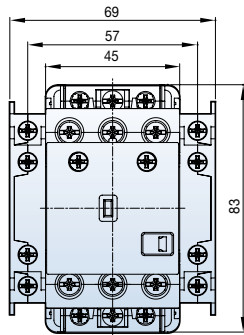
MC-32a~40a AC 2NO2NC + ML-65
