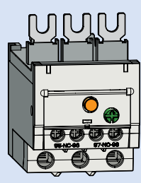
Overload relay, MT directly mountable to MC type contactor ▶ 94 page
