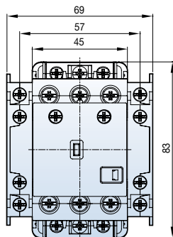
MC-32a~40a DC 2NO2NC + ML-65
