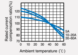
Temperature curve
