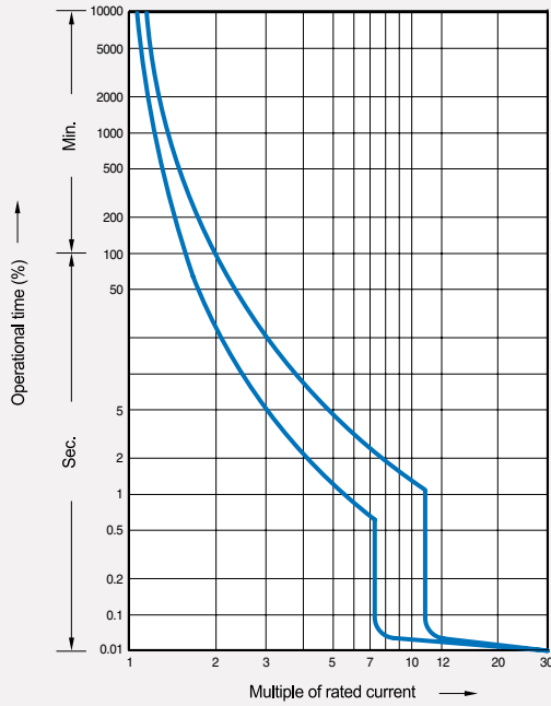
Operating curves
