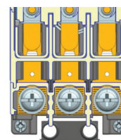
Dual Exhaust Structure - Indirect Arc Discharge
